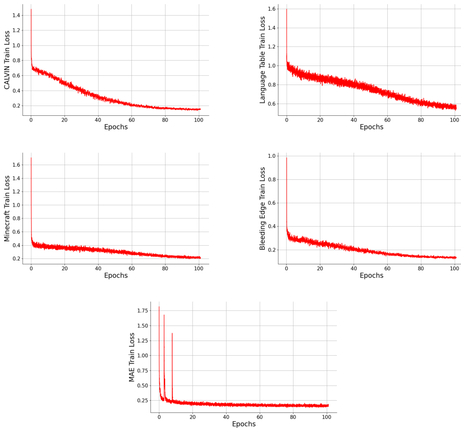
Figure 11. Plot of all components of the training loss over the 100 epochs of pre-training.
